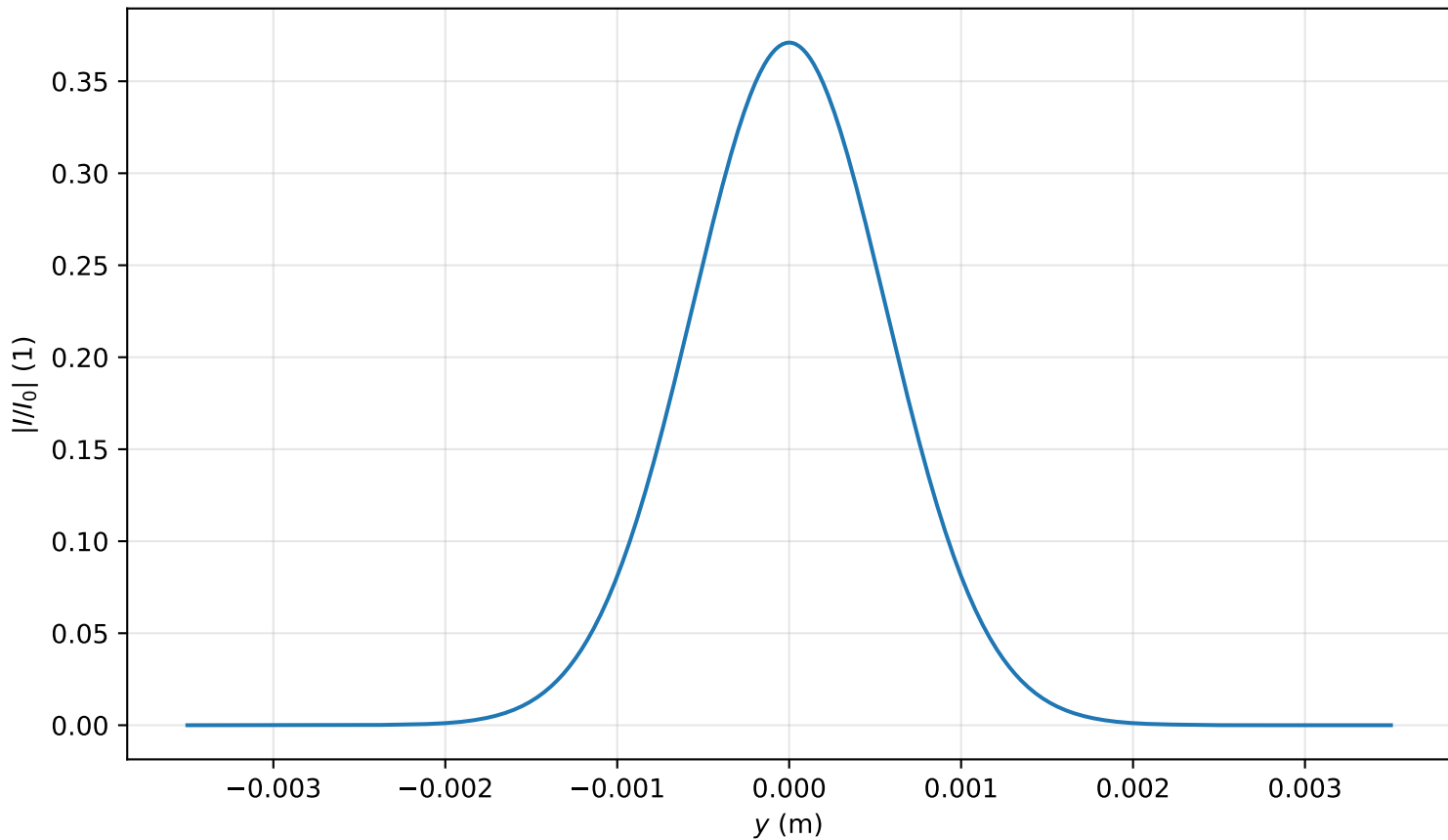
Intensity profile I(x=0, y, z=2.786)/I_0 , P_{in}=0.1P_{cr} , artificial time
